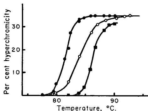
FIGURE 1 Melting-out curves of trout sperm (○), T2 (●), and T7 (■) bacteriophage DNA preparations in 0.15 M sodium chloride, 0.015 M sodium citrate.
